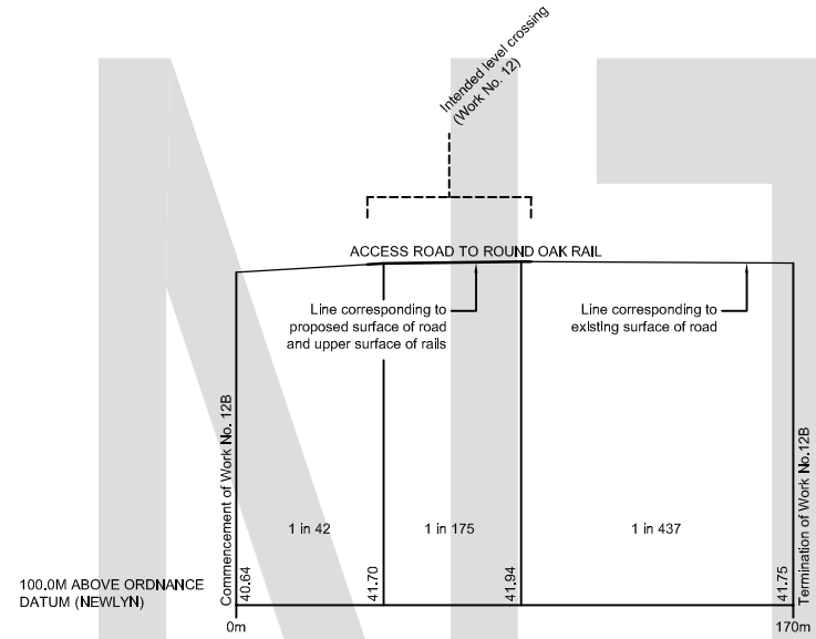
WORK No. 12B Alteration of access Road to Round Oak Rail (Gradient unaltered)
