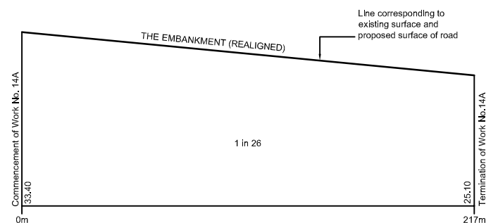
WORK No. 14A The Embankment (realignment)
