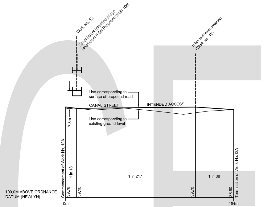
WORK No. 12A Canal Street extension
