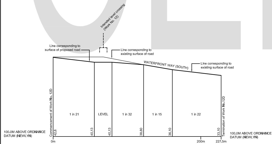
WORK No. 12D Alteration of Waterfront Way (South)
