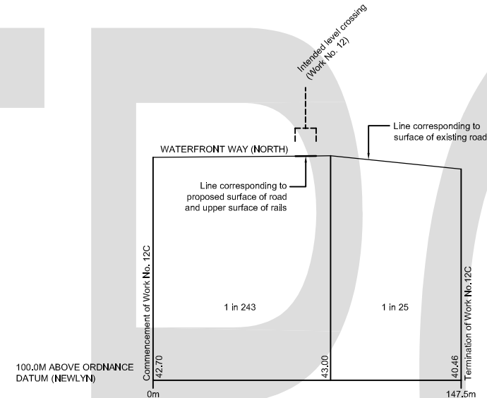
WORK No. 12C Alteration of Waterfront Way (North) (Gradient unaltered)
