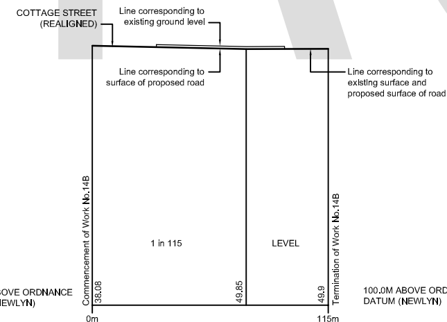
WORK No. 14B Cottage Street realignment
