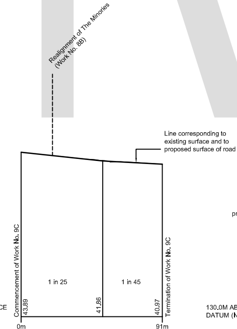
WORK No. 9C Constitution Hill extension
