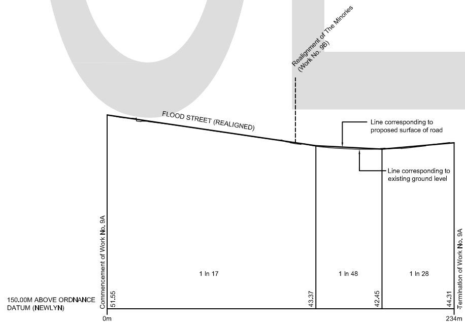
WORK No. 9A Flood Street realignment
