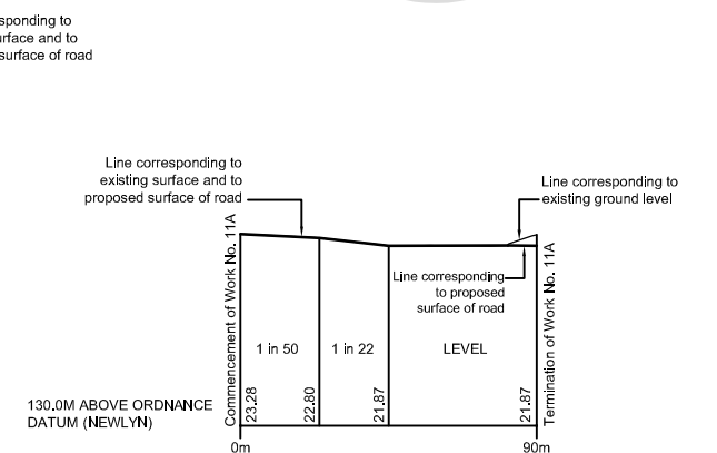
WORK No. 11A Pedmore Road tramstop access road from Buxton Road
