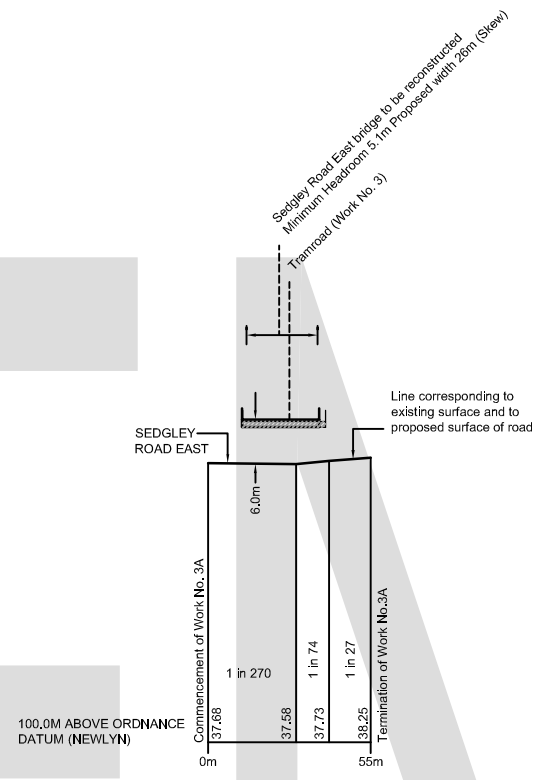
WORK No. 3A Sedgley Road East bridge reconstruction and widening
