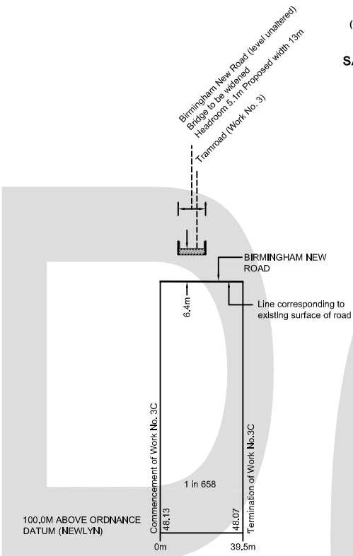
WORK No. 3C Birmingham New Road bridge widening
