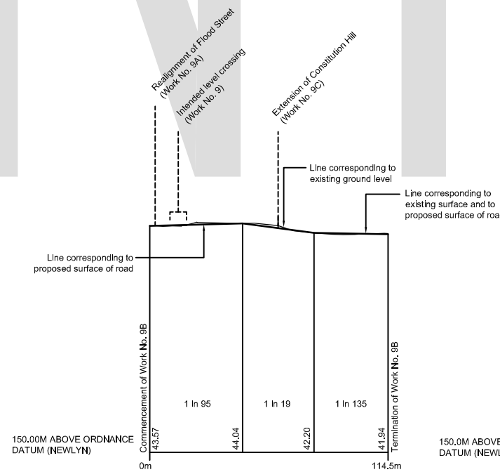
WORK No. 9B The Minories realignment
