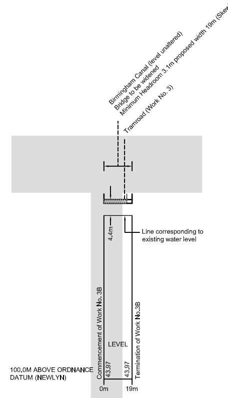
WORK No. 3B Birmingham Canal bridge widening
