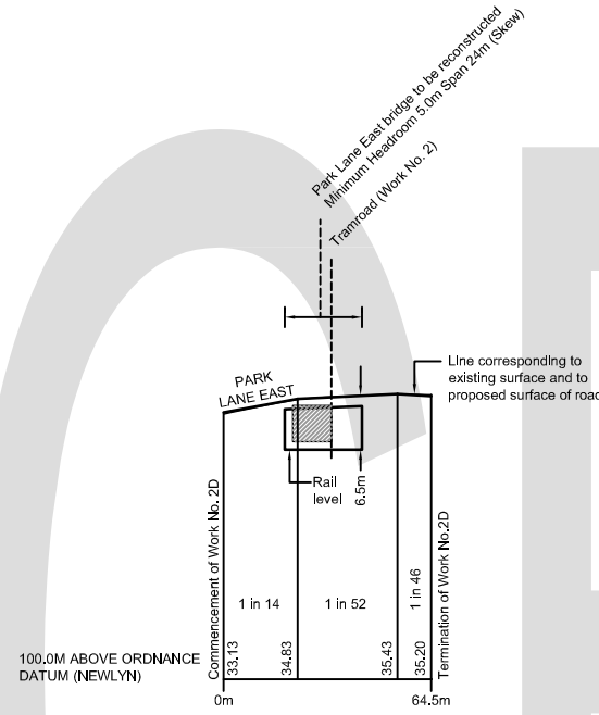
WORK No. 2D Park Lane East bridge reconstruction and widening
